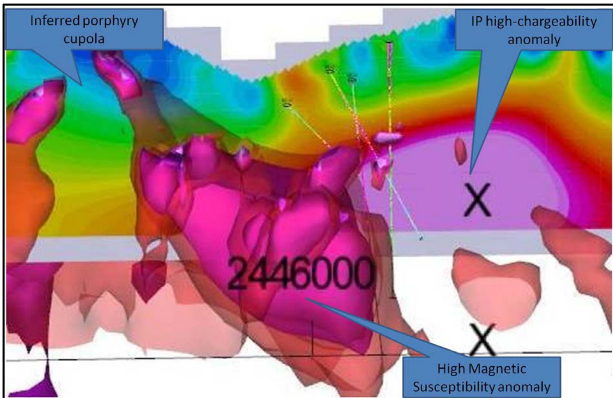
Figure 1 – Vertical east-west view of Cerro Blanco 3-D Magnetic Susceptibility 0.5, 0.6 & 0.7 S.I shells indicating possible porphyry cupola arch, with vertical slice of IP chargeability at 6460200N through drill-holes. Graphic shows apparent displacement of high magnetic susceptibility zones with respect to high IP chargeability zone.
